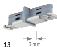
Isolator max. 2×2.000 W 230 V ⌀18 ⇄ 68 ⇄ 18 mm 951.47
