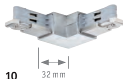
L-Connector max. 2×2.000 W 230 V ⌀18 ⇄ 66 ⇄ 66 mm 951.42
