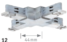
X-Connector max. 2×2.000 W 230 V ⌀18 ⇄ 112 ⇄ 112 mm 951.44
