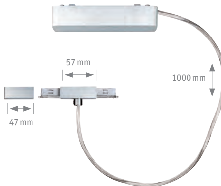
Wire Feed max. 2×2.000 W 230 V ⌀37 ⇄ 165 ⇄ 81 mm 951.35
