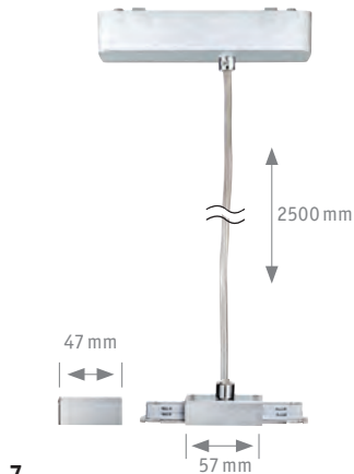
Suspension Feed max. 2×2.000 W 230 V ⌀37 ⇄ 165 ⇄ 81 mm 951.39
